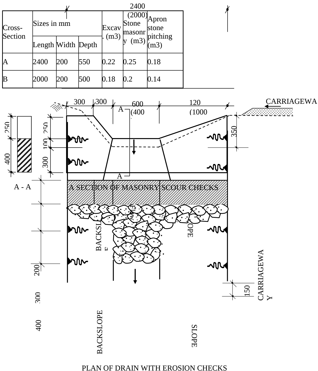
FIGURE C.6 - MASONRY SCOUR CHECKS
