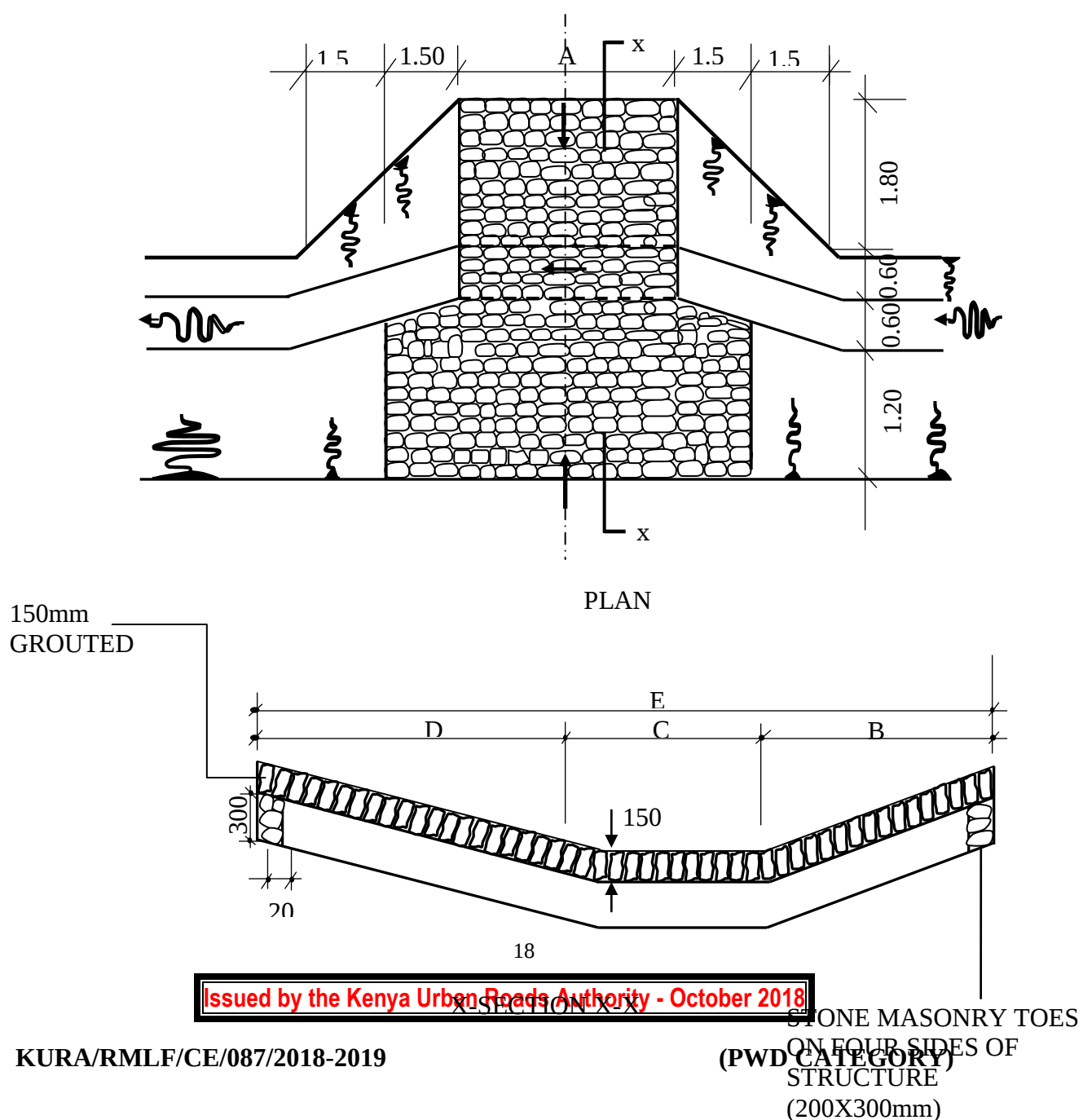
FIGURE C.15 ACCESS DRIFT
