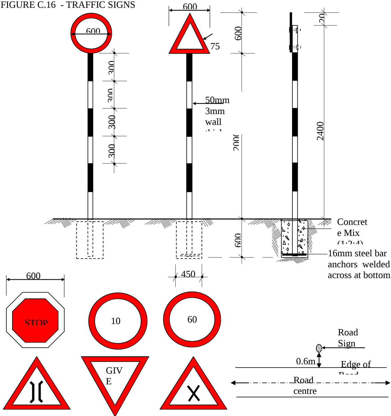
FIGURE C.16 - TRAFFIC SIGNS
