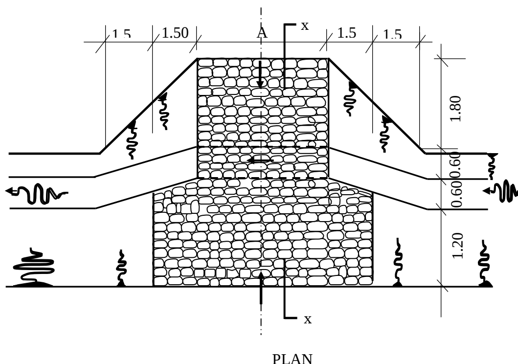
FIGURE C.15 ACCESS DRIFT
