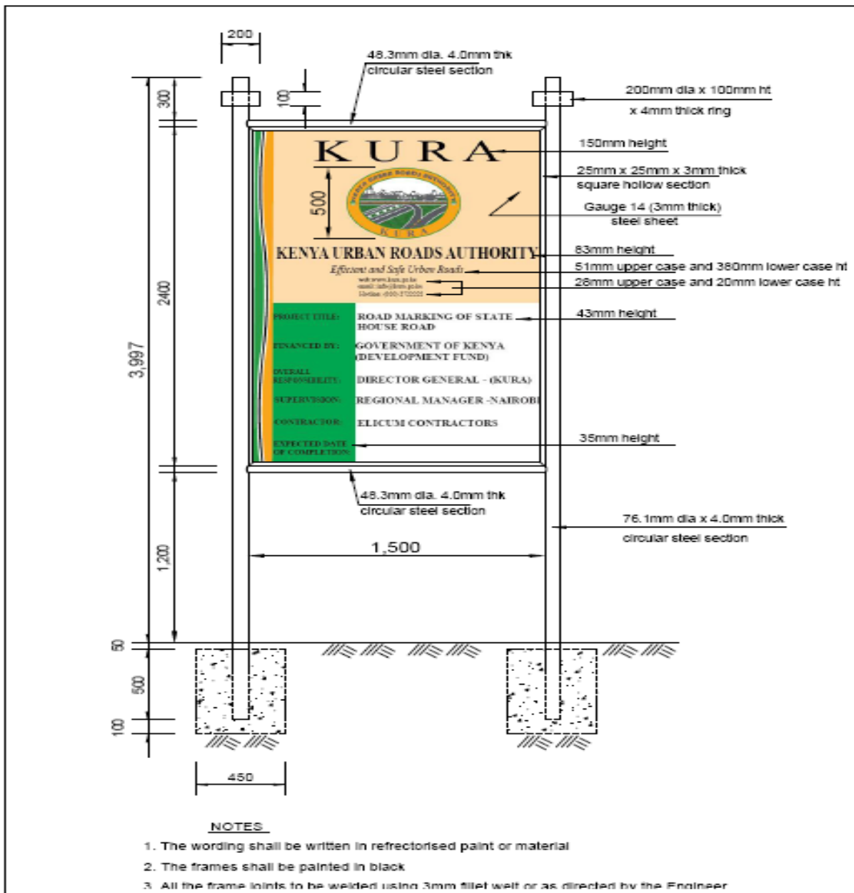
FIGURE 1 ~ PUBLICITY SIGN
