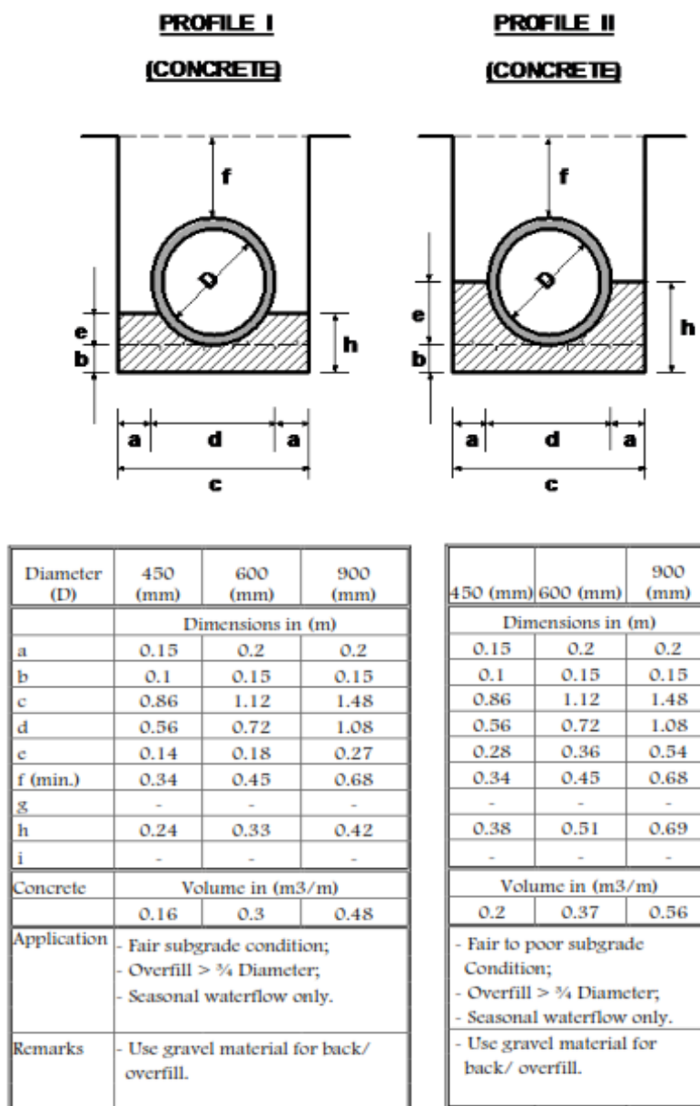
FIGURE C.7- BEDDING AND HAUNCH PROFILES TYPES I & II
