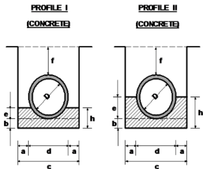
FIGURE C.7- BEDDING AND HAUNCH PROFILES TYPES I & II
