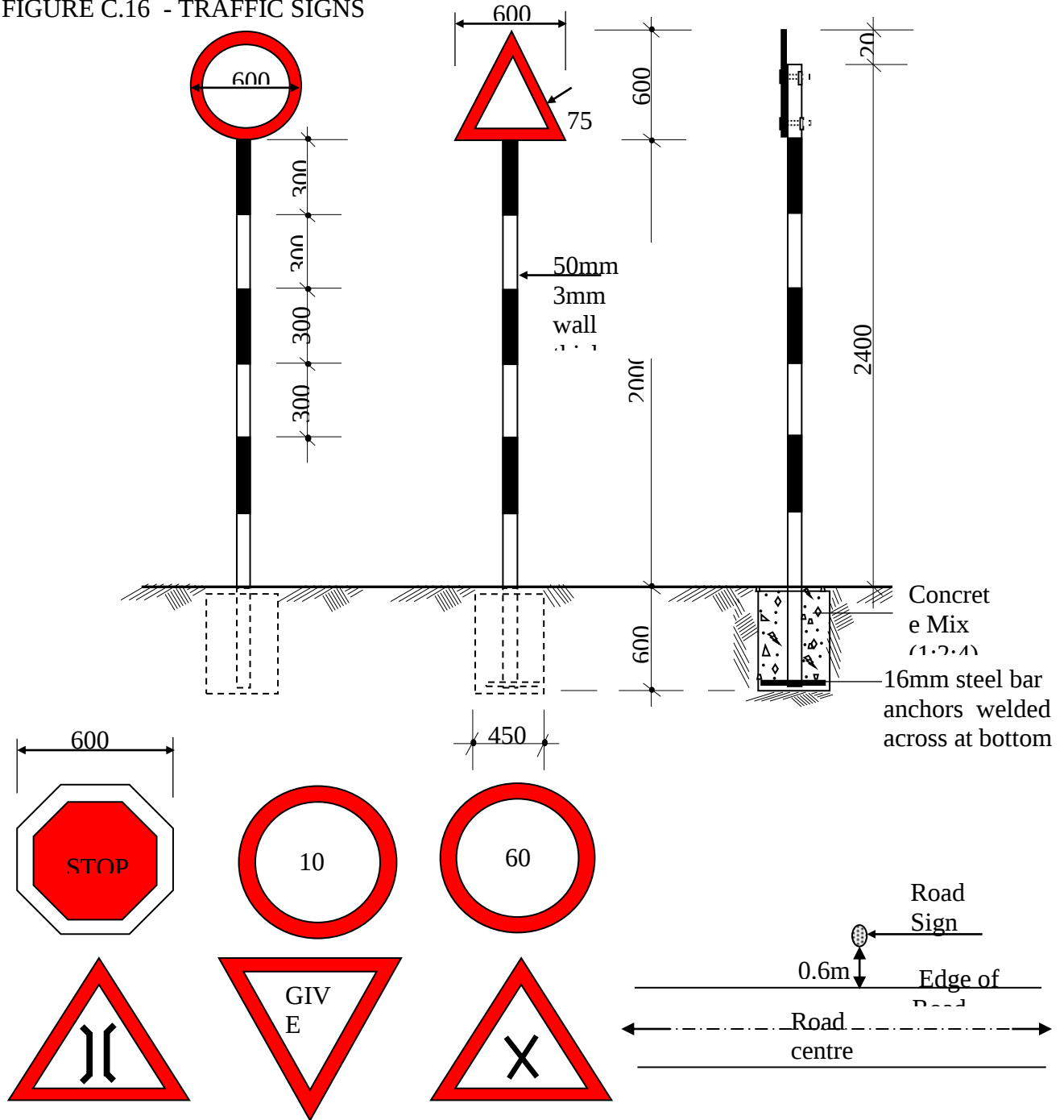
FIGURE C.16 - TRAFFIC SIGNS
