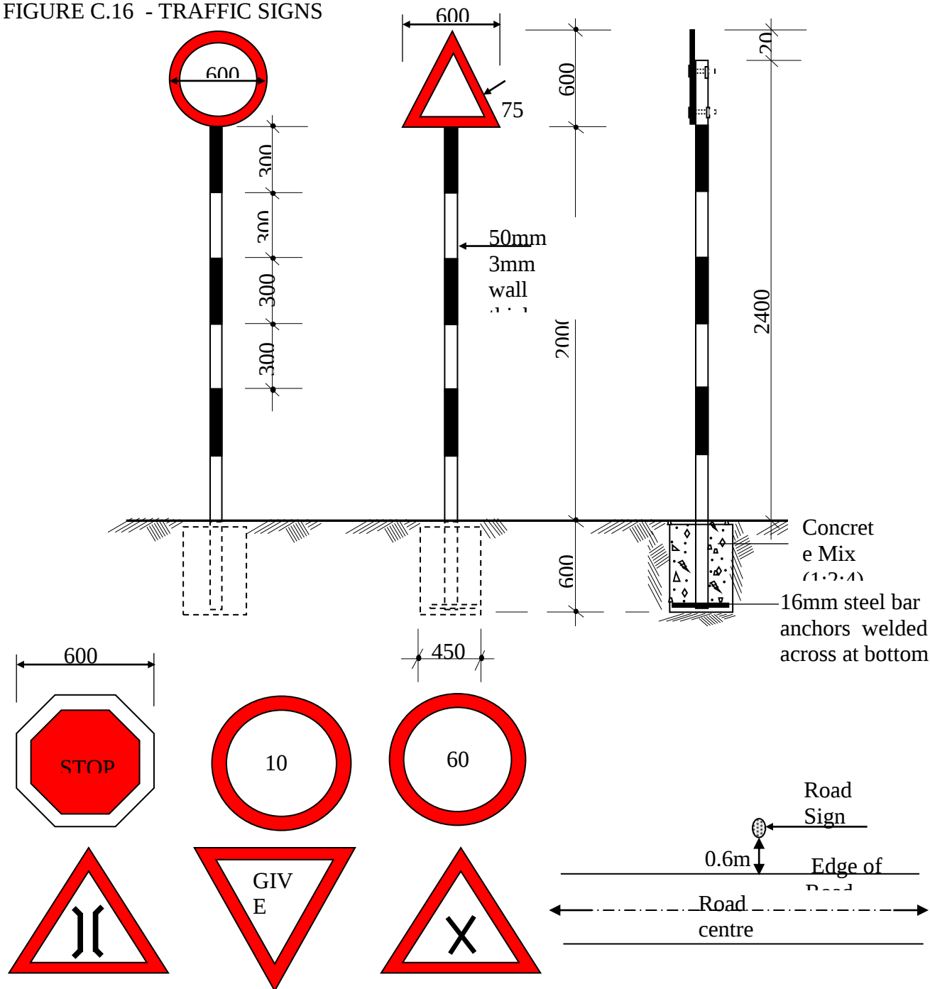
FIGURE C.16 - TRAFFIC SIGNS
