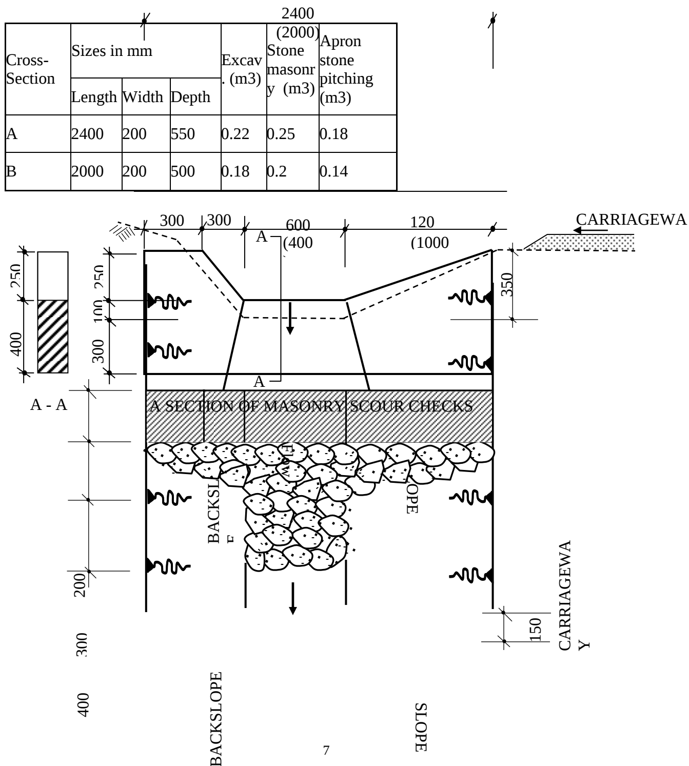
FIGURE C.6 - MASONRY SCOUR CHECKS
