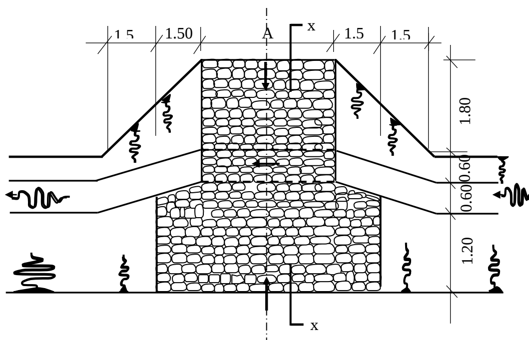
FIGURE C.15 ACCESS DRIFT
