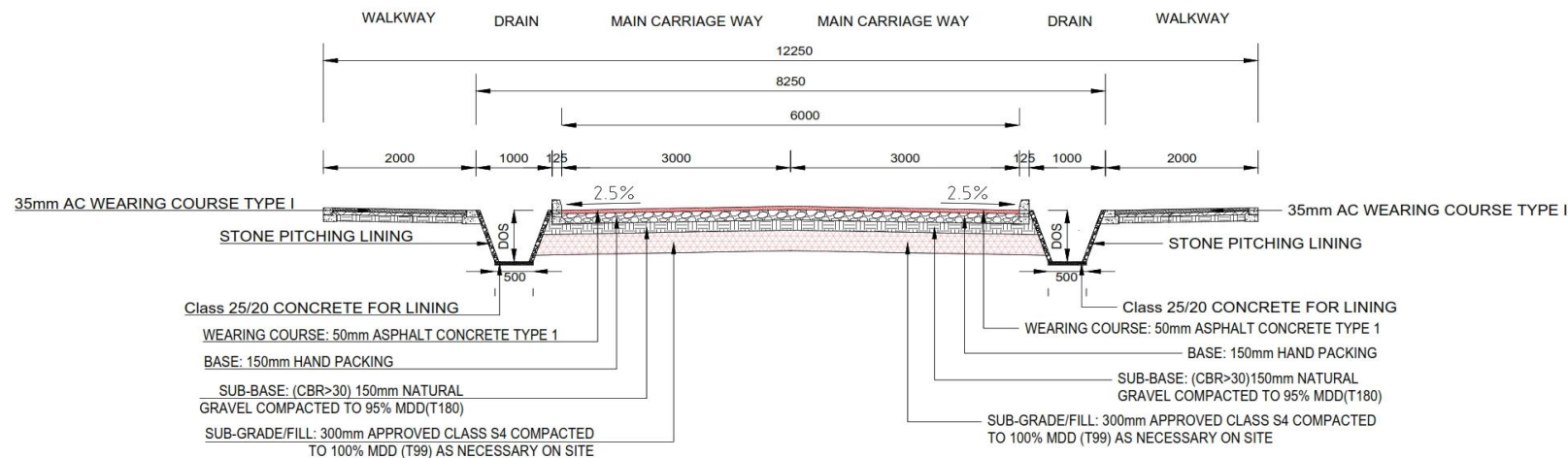
TYPICAL ROAD CROSS SECTION SCALE 1:30
