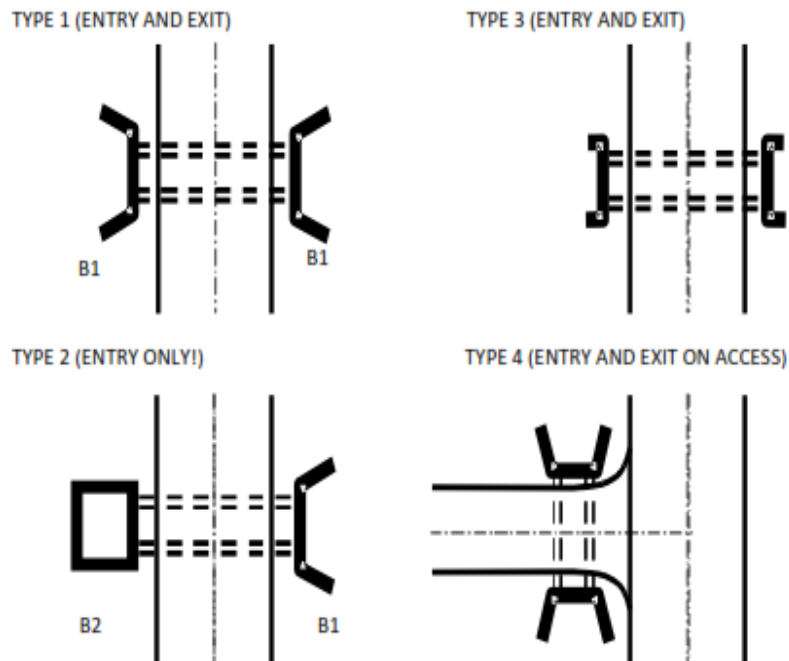
FIGURE C.1 - CULVERT ENTRY / EXIT STRUCTURE TYPES
