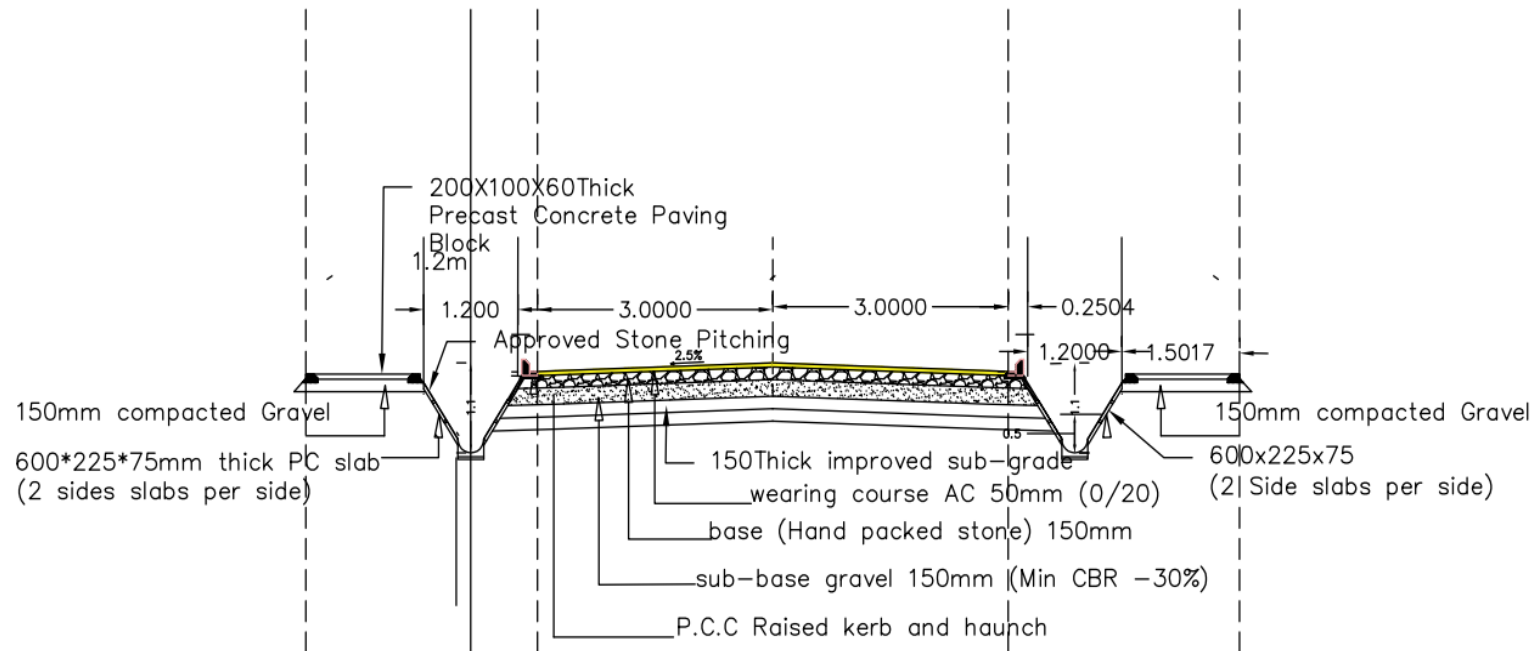
TYPICAL ROAD CROSS-SECTION
