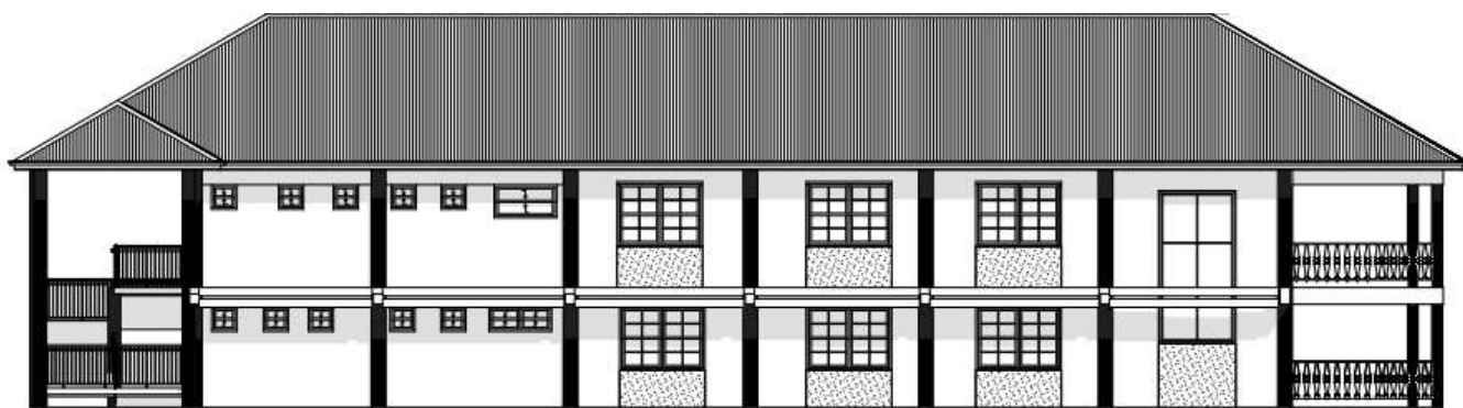
ELEVATION E-01
