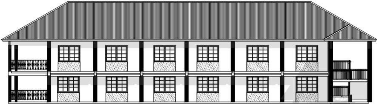
ELEVATION E-03
