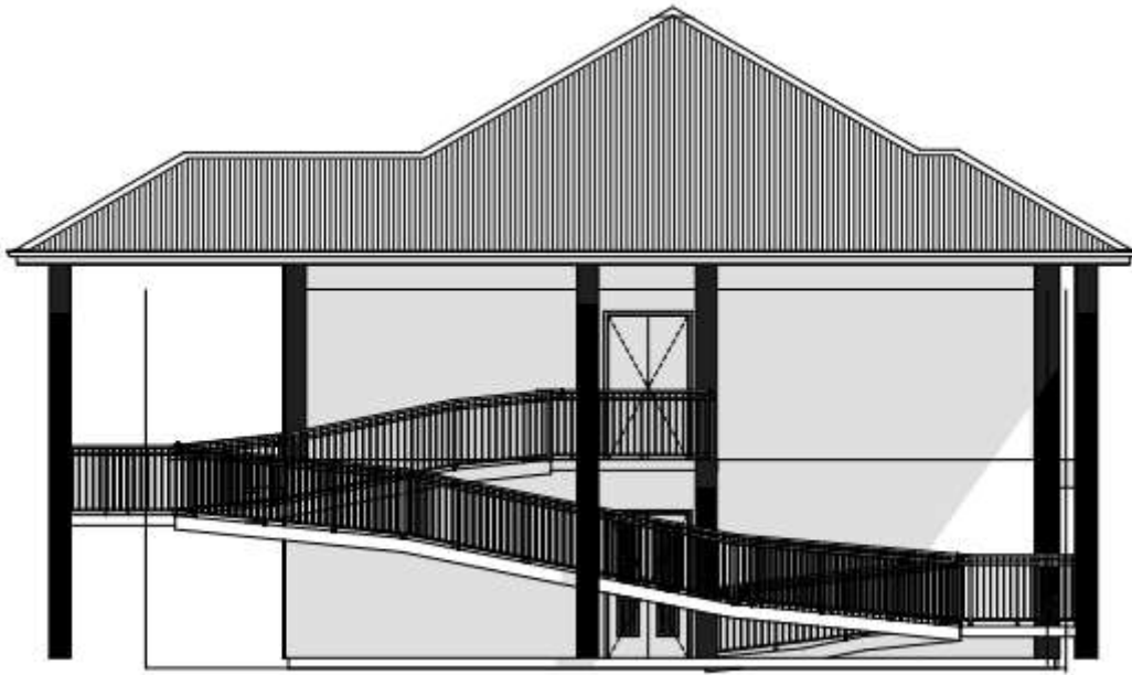
ELEVATION E-02
