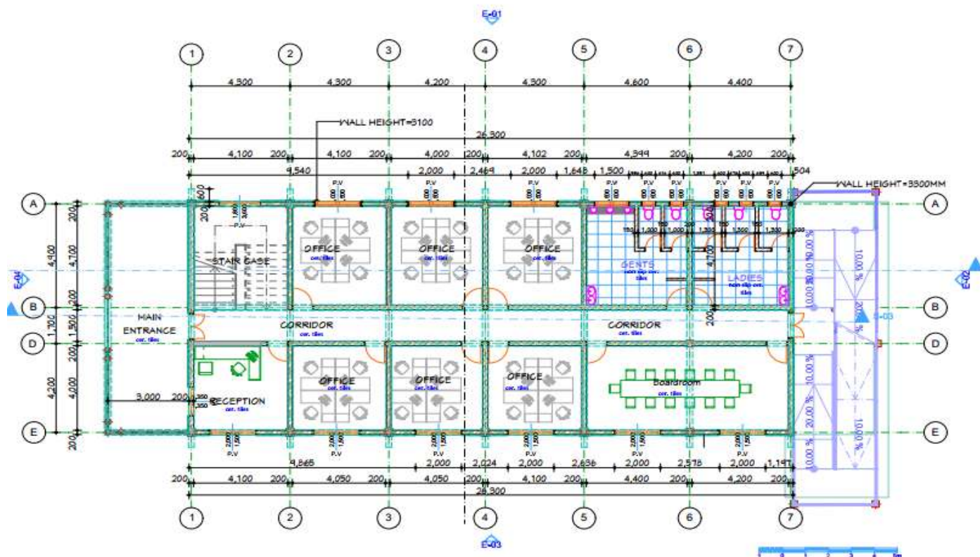
STOREY PLAN
