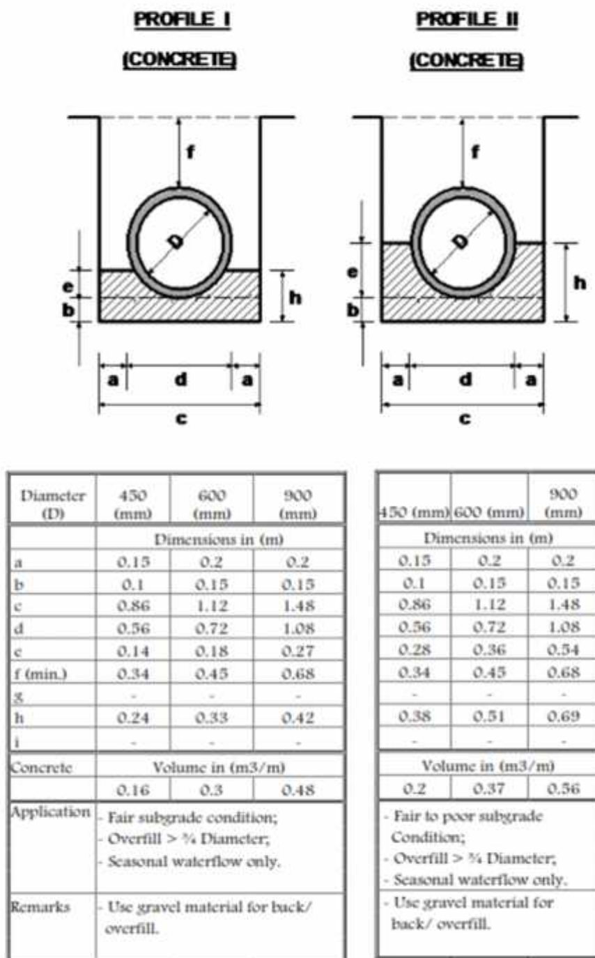
FIGURE C.7- BEDDING AND HAUNCH PROFILES TYPES I &amp; II
