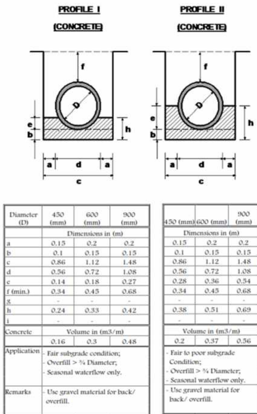
FIGURE C.7- BEDDING AND HAUNCH PROFILES TYPES I & II
