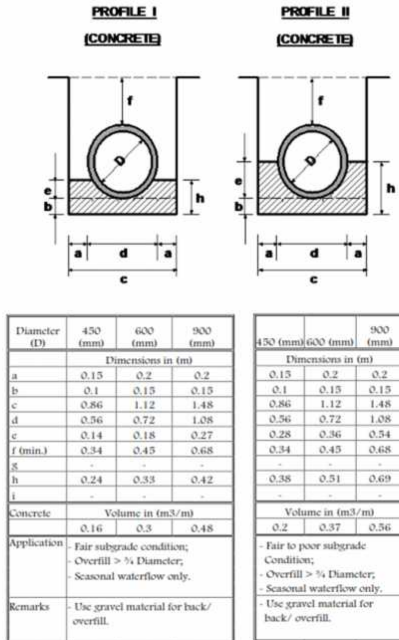
FIGURE C.7- BEDDING AND HAUNCH PROFILES TYPES I &amp; II
