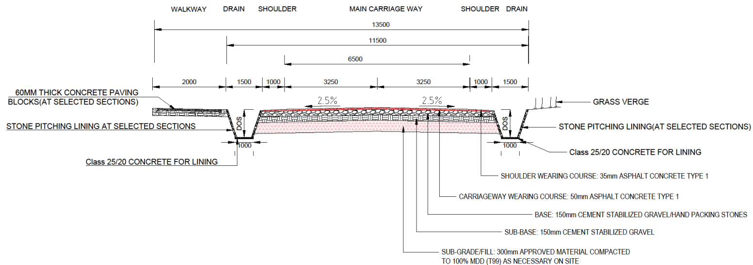
TYPICAL ROAD CROSS SECTION SCALE 1:30
